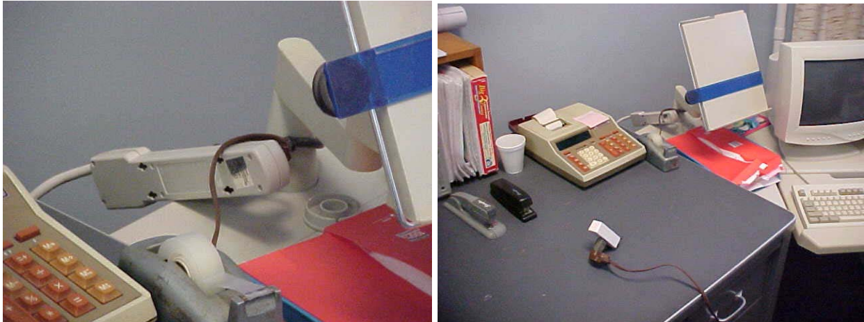
A potential tragedy in a Maine town office. A multiple outlet strip with a “zip cord” extension cord, ground “cheater”, and triple outlet adaptor. Depending on the appliances plugged into this setup, it could pose both a serious fire and electrocution hazard!
